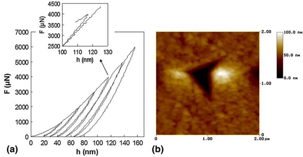
Fig. 5 (a) Cyclic nanoindentation curve performed on CrN coated \text{Zr}_{50}\text{Cu}_{40}\text{Al}_{10} at loading rate of 500 \mu\text{N/s} (b) AFM image of the obtained imprint after nanoindentation test
