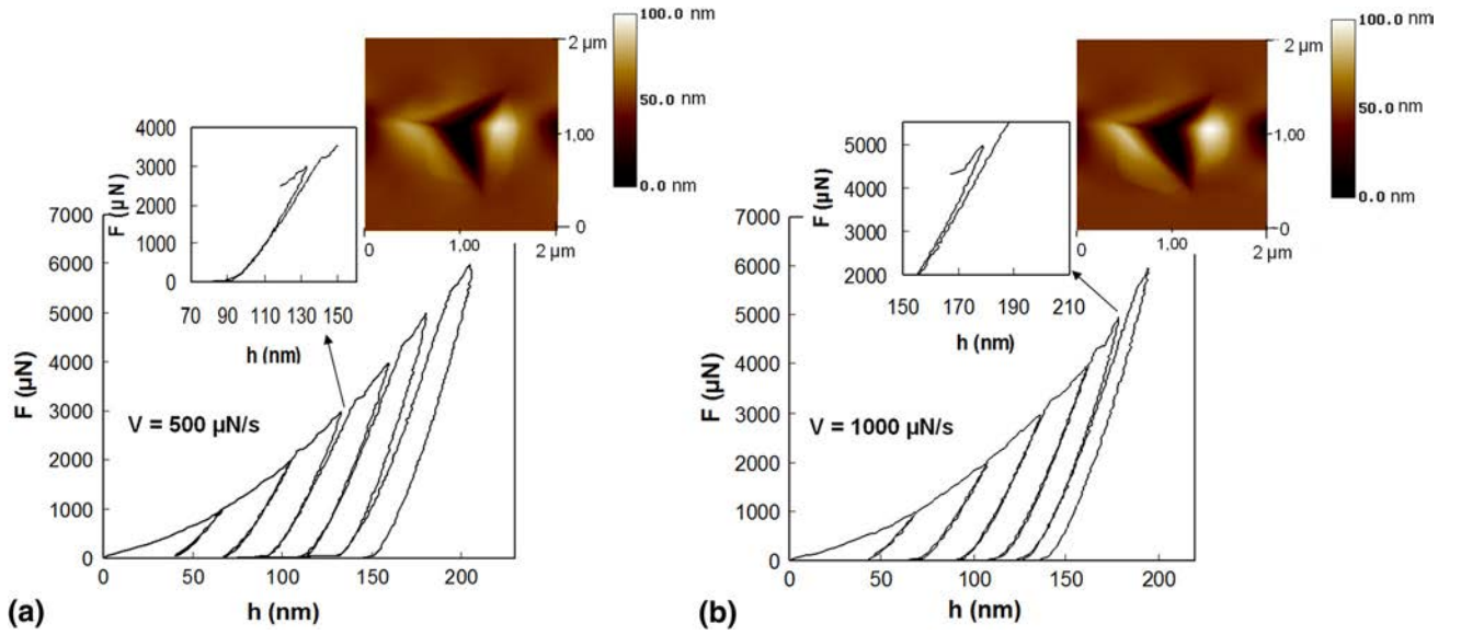
Fig. 2 Cyclic nanoindentation curves performed on \text{Zr}_{60}\text{Ni}_{10}\text{Cu}_{20}\text{Al}_{10} at loading rates of (a) 500 \mu\text{N/s} and (b) 1000 \mu\text{N/s}
