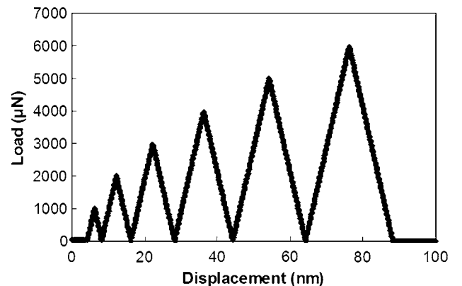
Fig. 1 Typical load vs. time function in cyclic nanoindentation tests (incremental cyclic loading) using Hysitron nanoindenter
