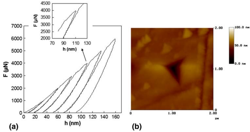
Fig. 3 (a) Cyclic nanoindentation curve performed on TiN coated \text{Zr}_{60}\text{Ni}_{10}\text{Cu}_{20}\text{Al}_{10} at loading rate of 500 \mu\text{N/s} (b) AFM image of the obtained imprint after nanoindentation test
