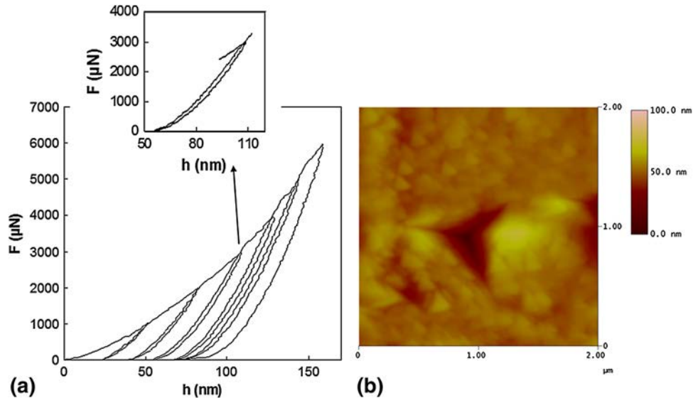
Fig. 4 (a) Cyclic nanoindentation curve performed on Ti/TiN coated \text{Zr}_{60}\text{Ni}_{10}\text{Cu}_{20}\text{Al}_{10} at loading rate of 500 \mu\text{N/s} (b) AFM image of the obtained imprint after nanoindentation test
