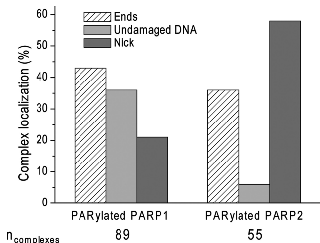
Figure 7. AFM analysis of the position distributions of PARylated PARP1(2) on nicked 1200-bp DNA. PARP1 (3.5 nM) or PARP2 (3.5 nM) was incubated with 1200-bp nicked DNA (1.5 nM) at 37°C for PARP1 and on ice for PARP2 for 60 min in the presence of 100 \mu M NAD + . Number of complexes analysed: 89 for PARP1 and 55 for PARP2.
