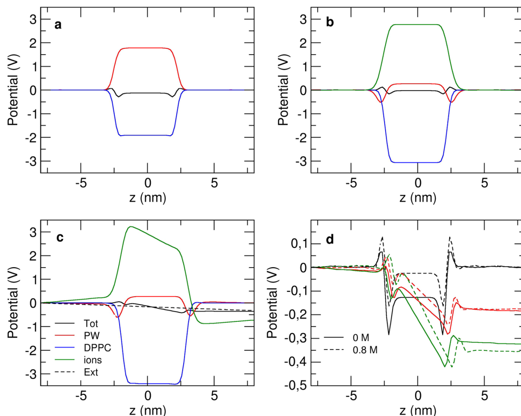
Figure 3. (a–c) Total electric potential along the z axis of a CG DPPC membrane (black) and its decomposition, without ions (a), with 0.8 M ionic concentration (b), with no external electric field, and in the presence of an external electric field of 0.02 V/nm (c). (d) Total electrostatic potentials with no electric field (black), electric fields of 0.01 V/nm (red) and 0.02 V/nm (green) without ions (solid line) and with 0.4 M and 0.8 M concentrations (dashed lines).
