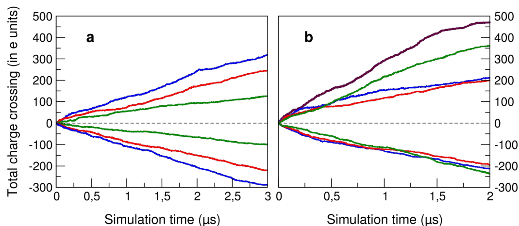
Figure 5. Cumulative current as a function of time, for potentials (a) under or (b) over 300 mV computed during 3 or 2 \mu s, respectively. (a): \pm 92 mV (green), \pm 185 mV (red) and \pm 277 mV (blue). (b): \pm 370 mV (green), \pm 462 mV (red), \pm 555 mV (blue) and \pm 740 mV (violet).
