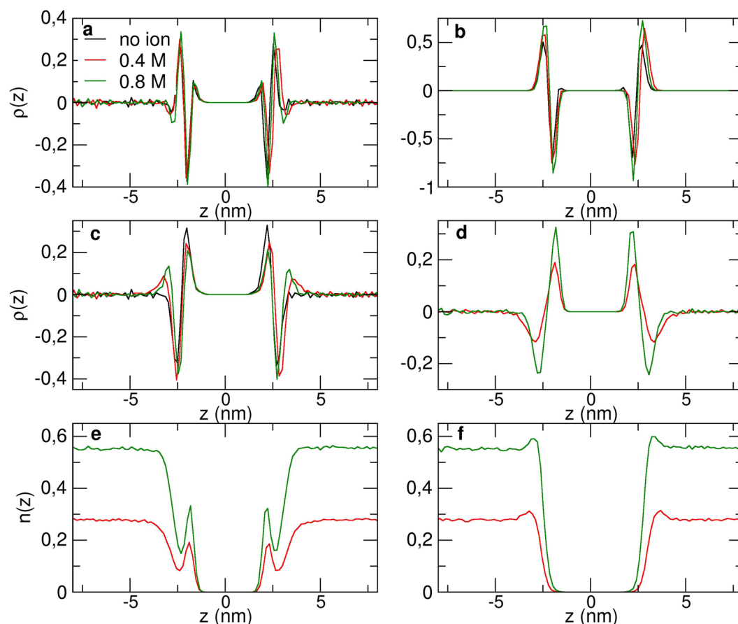
Figure 2. (a) Total linear charge density along the z axis around a CG DPPC bilayer with (0.4 M in red and 0.8 M in green) and without ions (in black), and its decomposition: (b) DPPC charge density, (c) solvent, (d) ions. (e–f): Particle density for K^+ (e) and Cl^- (f) ions. The z axis is centered at the middle of the lipid bilayer.
