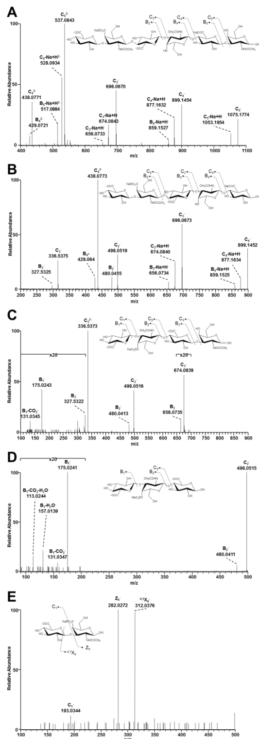
Figure 6. Negative nanoESI sequential fragmentations of the synthetic A-A-A ion at m/z 632.6847 after sulfatase action during 24 h. (A) MS 2 spectrum of the [dp6-2SO 3 -4Na+2H] 2- precursor ion at m/z 632.6847, (B) MS 3 spectrum of the C 5 2- ion at m/z 537.0843, (C) MS 4 spectrum of the C 4 2- ion at m/z 438.0773, (D) MS 5 spectrum of the C 3 - ion at m/z 336.5373 and (E) MS 6 spectrum of the C 2 - ion at m/z 498.0515.
