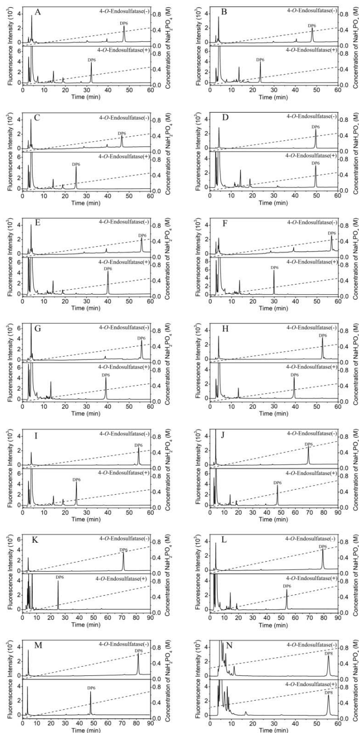
FIGURE 2. Analysis of the final products of CS/DS oligosaccharides digested with 4- O -endosulfatase. Unsaturated CS/DS oligosaccharides of CS-A3 (A), CS-A4 (B), CS-A5 (C), CS-A7 (D), CS-A9 (E), CS-A10-1 (F), CS-A10-2 (G), CS-A10-3 (H), CS-A11(I), CS-E7 (J), CS-E9 (K), CS-E13 (L), CS-E15 (M) and octasaccharide (N) were exhaustively digested without (top) or with (bottom) 4- O -endosulfatase, labeled with 2-AB, and then analyzed by anion exchange HPLC as described under “Experimental Procedures.”
