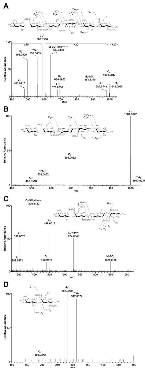
Figure 4. Negative nanoESI sequential fragmentations of the synthetic A-A-A ion at m/z 689.5937 after sulfatase action during 3 h. (A) MS 2 spectrum of the [\text{dp6-SO}_3\text{-3Na+H}]^{2-} precursor ion at m/z 689.5937, (B) MS 3 spectrum of the \text{C}_5^{2-} ion at m/z 588.0510, (C) MS 4 spectrum of the \text{C}_4^- ion at m/z 1001.0842 and (D) MS 5 spectrum of the \text{C}_2^- ion at m/z 498.0513.
