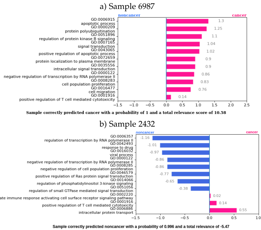
Figure 3: Explanation of (a) a cancer and (b) a noncancer prediction. A subset of eleven GO terms is reported with their relevance score and their description. The color indicates towards which class a GO term influences the signal: blue for noncancer and pink for cancer. The total relevance score is the sum of the relevance scores and the bias of the output class.
