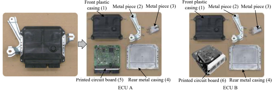
Figure 1: The example of two Toyota Vitz ECUs (Environmental Affairs Division, 2017)
