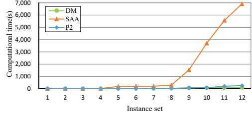
(b) Computational time
