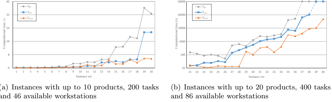
Figure 12: Comparison with P3 and the classic CS method
