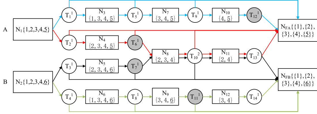
Figure 2: Disassembly schemes of products A and B
