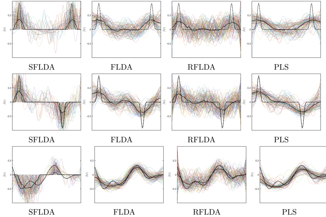
Figure 2: Discriminant functions from 100 repetitions of the simulation study estimated by SFLDA, FLDA, RFLDA, and PLS, for Settings 1, 3, and 5. The thicker black line in each plot represents the median of the estimated curves, while the dot-dashed curve is the true discriminant function.
