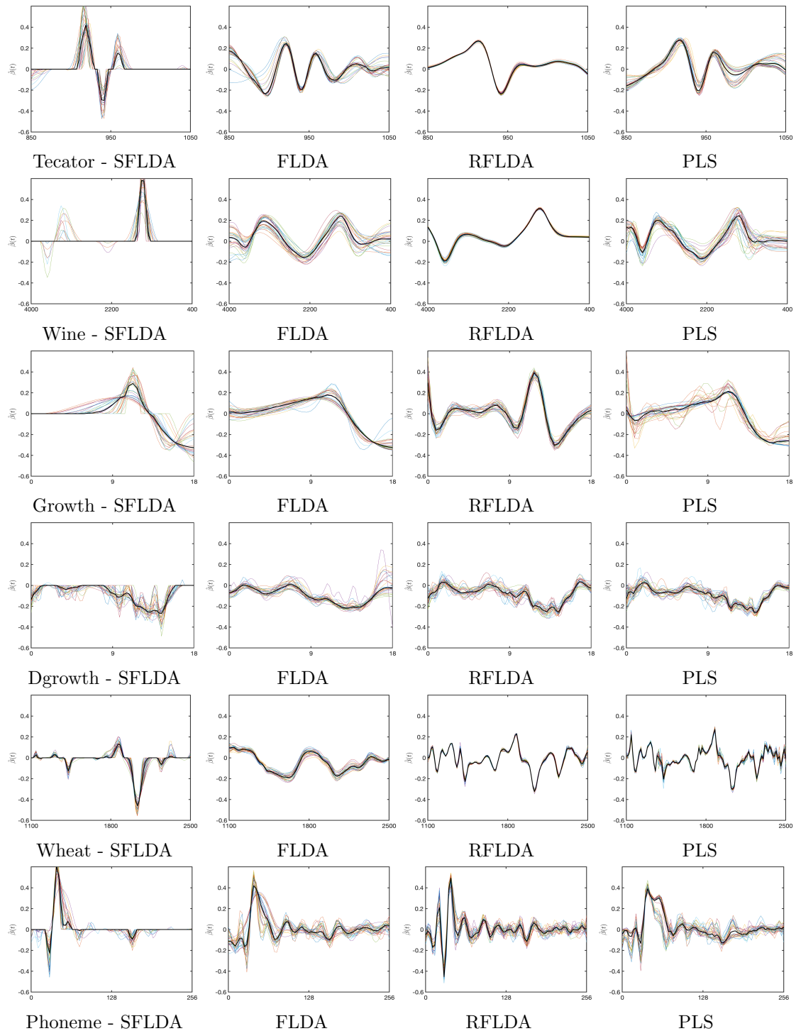
Figure 4: Estimated discriminant curves for real data examples from 30 repetitions. The median curve is shown as a thicker black solid line.
