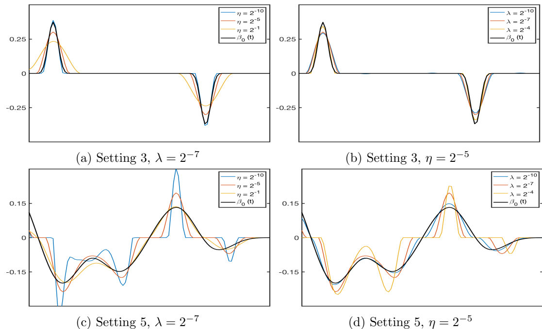
Figure 1: Illustration of the roles of the tuning parameters \eta and \lambda . Each panel plots the true \beta_0(t) , as well as \tilde{\beta}(t) with a varying tuning parameter.
