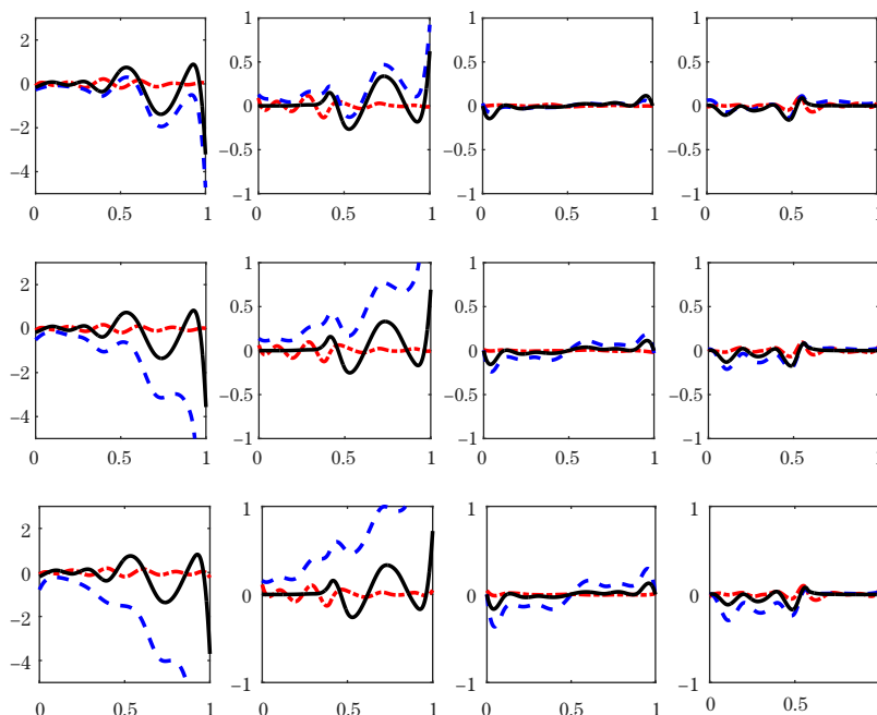
Figure 5. Comparison of the bias of the nonzero coefficient functions \beta_1, \beta_2, \beta_3, and \beta_4 (from left to right) based on the LSE (dot-dashed), LASSO (dashed), and PLSE_{0.5} (solid), for p = 5 (top row), p = 20 (middle), and p = 50 (bottom) in Scenario 3.
