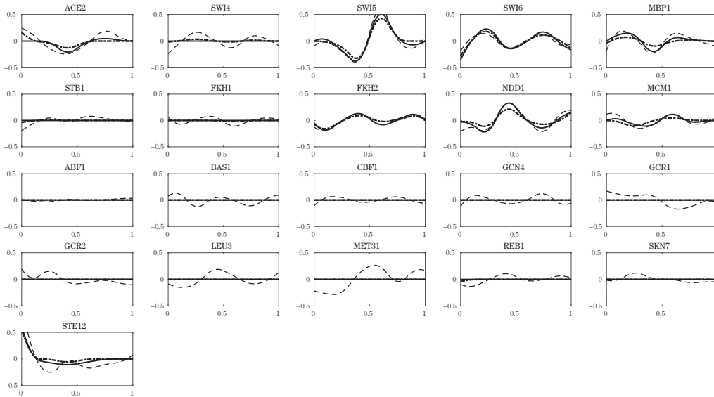
Figure 8. Subplots of estimated coefficient functions for the 21 confirmed TFs using the LSE (dashed), LASSO (dot-dashed), and PLSE_{0.5} (solid).
